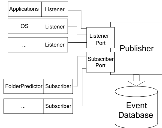
Figure 2. Publisher-Subscriber Architecture.
